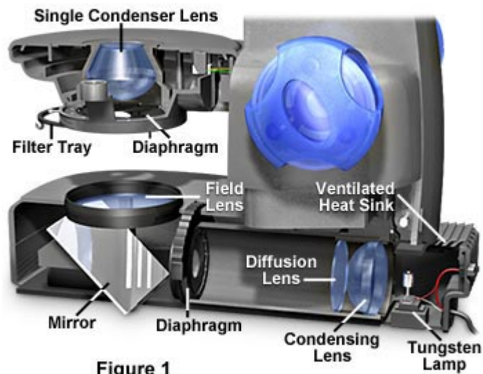
Figure 1 QX3 Aftermarket Illuminator Exploded Diagram
